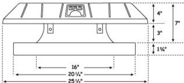
Curb Model – Side View
